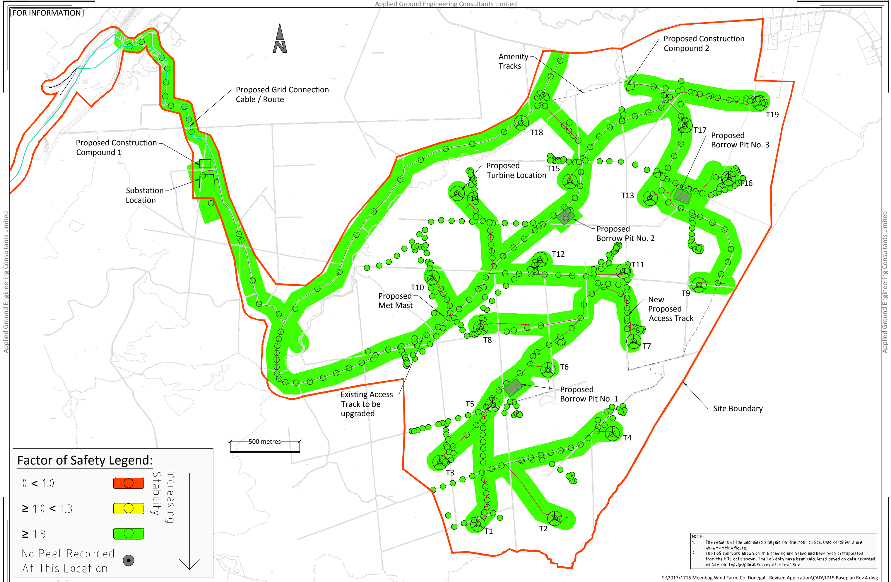
Figure 6 Factor of Safety Plan
