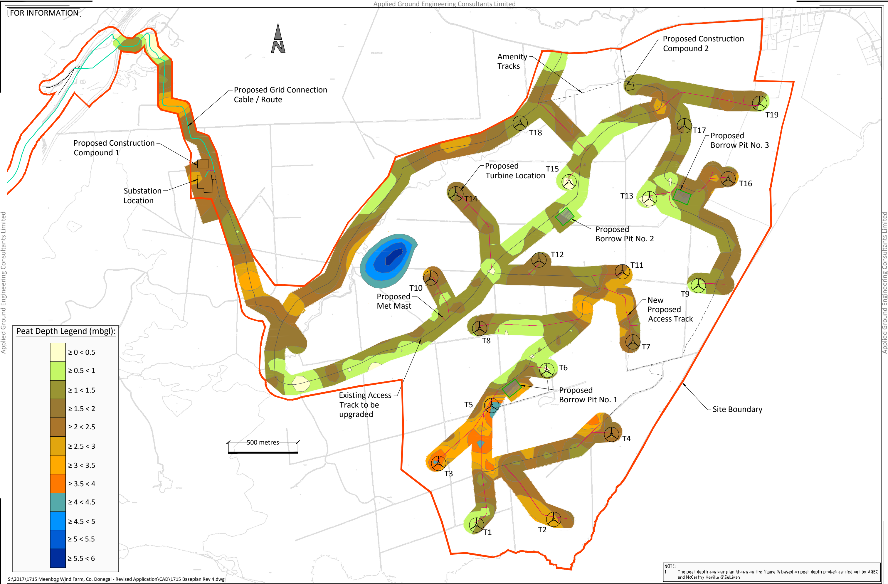
Figure 3 Peat Depth Contour Plan
