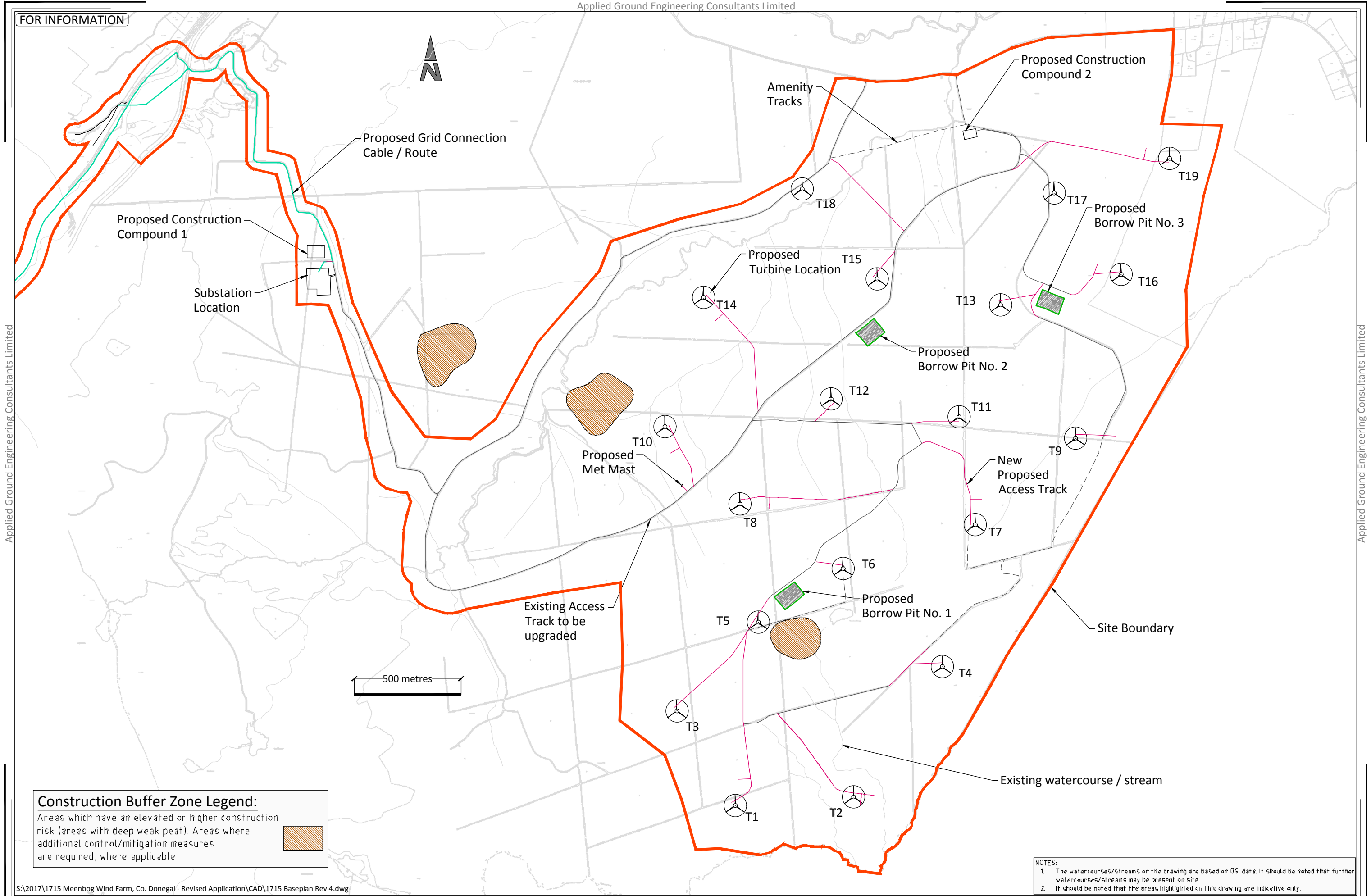
Figure 4 Construction Buffer Zone Plan
